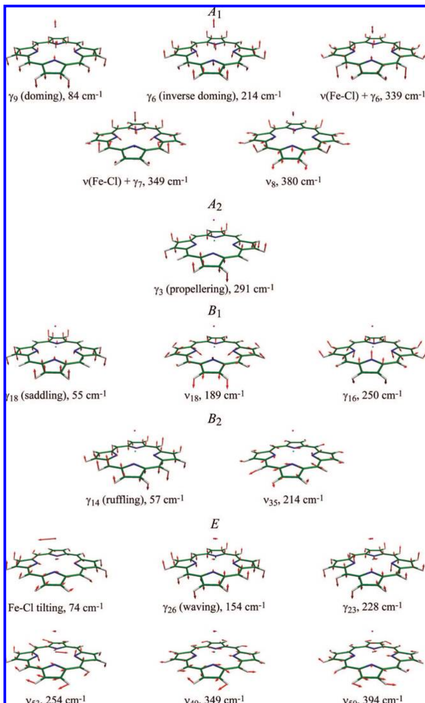
Figure 1. Normal vibrational modes of Fe(P)(Cl) below 400\text{ cm}^{-1} . The iron, chlorine, carbon, nitrogen, and hydrogen atoms are shown in light blue, pink, green, blue, and white, respectively. Eigenvectors are shown by red arrows.
