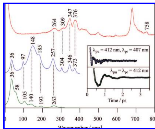
Figure 4. Correlations between Raman and coherence spectra for NP4-H 2 O at pH 5.6. Raman spectrum (red) was measured with excitation at 413.1\text{ nm} , whereas open band (green) and detuned (blue) coherence spectra were measured at a carrier wavelength of 412\text{ nm} . The detuned coherence data were collected with a 0.5\text{ nm} spectral window, detuned 5\text{ nm} to the blue of the carrier wavelength. (Inset) Time-domain oscillation data (circles) and LPSVD fits (lines) corresponding to an open band detection (green) and to a detuned detection (blue) scheme.
