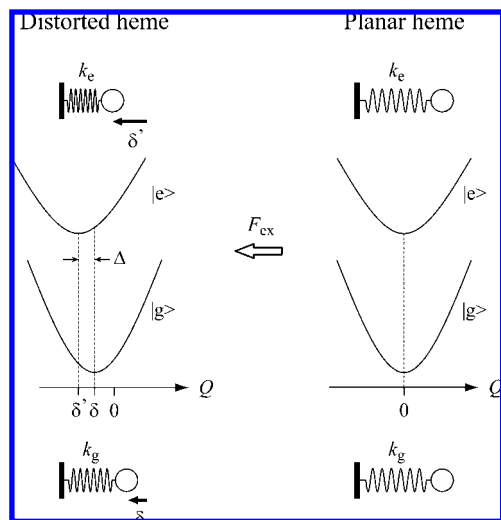
Figure 7. The compressed spring model for the “distortion-induced” Franck–Condon activity of OOP modes. In this model, the heme is distorted by the surrounding protein matrix and viewed as a spring compressed by an external force F_{\text{ex}} . The quantities k_g and k_e are the force constants of the mode Q in the ground and excited electronic states, respectively. The dimensionless equilibrium positions in the ground state \delta and in the excited state \delta' are proportional to F_{\text{ex}}/k_g and F_{\text{ex}}/k_e , respectively, and accordingly, the equilibrium position shift of the excited state relative to the ground state ( \Delta ) is obtained as \Delta = \delta' - \delta = \delta(k_g/k_e - 1) .
