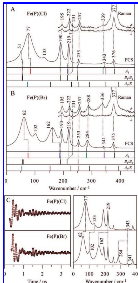
Figure 3. Comparison of experimental spectra and calculated frequencies for (A) Fe(P)(Cl) and (B) Fe(P)(Br). Polarized Raman spectra were measured with excitation at 413.1 nm, whereas open band coherence spectra were measured at a carrier wavelength of 412 nm. The calculated frequencies are categorized into 3 symmetry groups ( A 1 , B 1 / B 2 , and A 2 / E ) and are shown by bars. The calculation predicts frequency shifts for 4 A 1 modes and 1 E mode when Cl is exchanged with Br, where each mode is highlighted by a different color (red, blue, green, purple, and light blue). Correspondences between the Raman bands, FCS bands, and DFT frequencies are displayed by dotted lines. (C) Open-band coherence oscillation data, LPSVD fits (left) and LPSVD power spectra (right) of Fe(P)(Cl) and Fe(P)(Br). The frequency shifts between the two samples are displayed by dotted lines.
