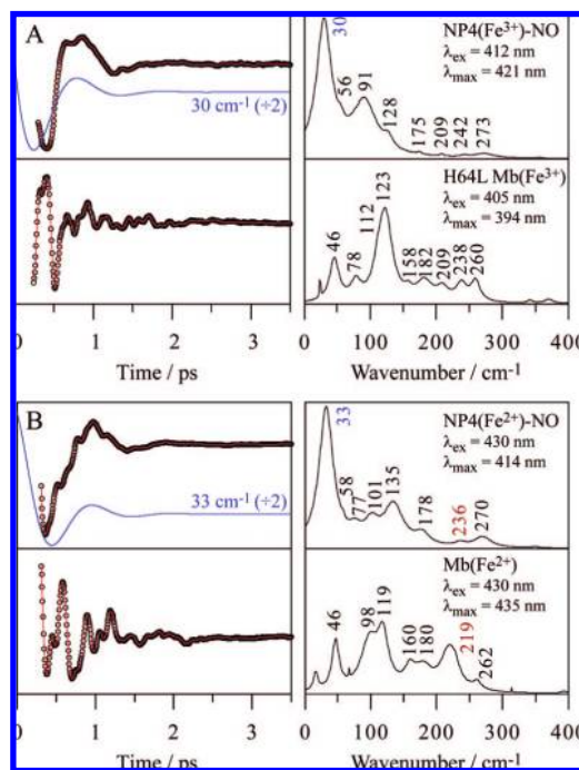
Figure 6. Open-band coherence oscillation data, LPSVD fits (left) and LPSVD power spectra (right) of (A) ferric NP4–NO and H64L Mb and (B) ferrous NP4–NO and Mb. The pH employed was 5.6 for the NP4–NO samples and 7.0 for the Mb samples. Acidic pH for NP4–NO was chosen to achieve a high geminate yield (~99%) of NO rebinding, which is required in the present FCS experiments using a high-repetition-rate laser. The excitation wavelengths are indicated in the right panels. The strong ~30 cm -1 (blue) oscillations of NP4 in the LPSVD fits are divided by a factor of 2 and shown in the left panel, displaced from the raw data for display purposes. The frequencies of \nu(\text{Fe-His}) of the ferrous species are shown in red.
