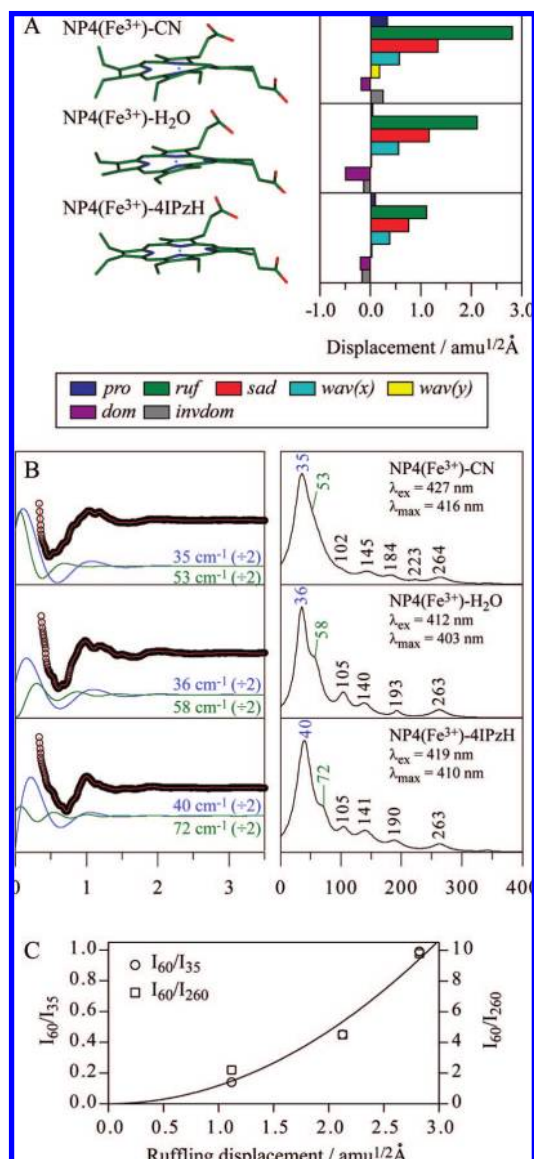
Figure 5. (A) Crystal structures and NSD analysis of hemes in ferric NP4–CN, NP4–H 2 O, and NP4–4IPzH. A displacement of 1 amu 1/2 Å represents that the square root of the sum of squares of the displacements of Fe and 24 porphyrin (4N, 20C) atoms is 1 amu 1/2 Å. The color coding for the modes is pro : propellering (blue), ruf : ruffling (green), sad : saddling (red), wav(x) : waving x (light blue), wav(y) : waving y (yellow), dom : doming (purple), invdom : inverse doming (gray). The minus sign of displacement is defined only for doming and inverse doming to indicate the direction of Fe displacement (+: proximal; -: distal). PDB IDs are 1EQD, 1D3S, and 1ML7 for NP4–CN, NP4–H 2 O, and NP4–4IPzH, respectively. (B) Open-band coherence oscillation data, LPSVD fits (left) and LPSVD power spectra (right) of ferric NP4–CN, NP4–H 2 O, and NP4–4IPzH. The pH was 5.6 for NP4–CN and NP4–H 2 O and 7.0 for NP4–4IPzH, which are consistent with the X-ray crystallographic studies. The excitation wavelengths are indicated in the right panels. The ~35 cm -1 (blue) and ~60 cm -1 (green) oscillations in the LPSVD fits are divided by a factor of 2 and shown in the left panel, displaced from the raw data for display purposes. (C) Intensity of the ~60 cm -1 band relative to the ~35 cm -1 and ~260 cm -1 bands. A solid line represents the least-squares-fitted quadratic curve passing through the origin (zero intensity at zero displacement).
